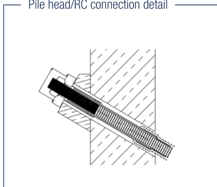
Pile head/RC connection detail
