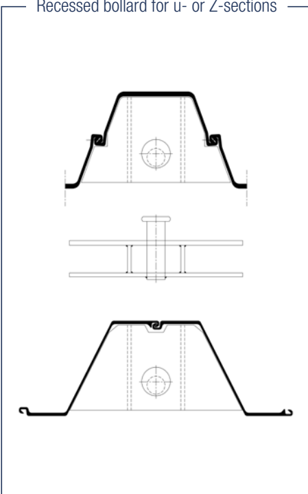
Recessed bollard for u- or Z-sections
