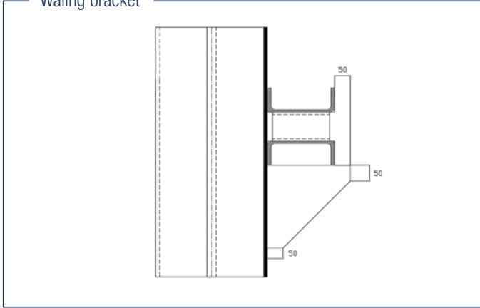
Suspended waling support
