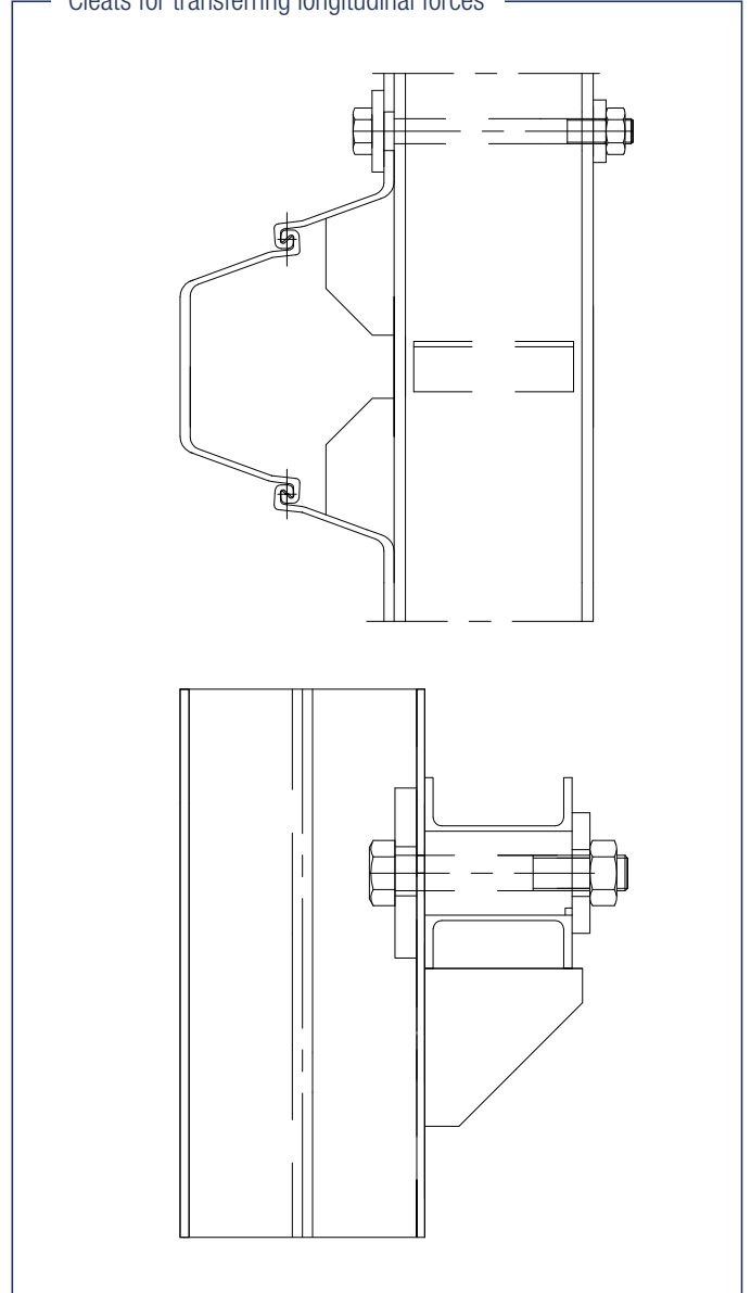
Cleats for transferring longitudinal forces
