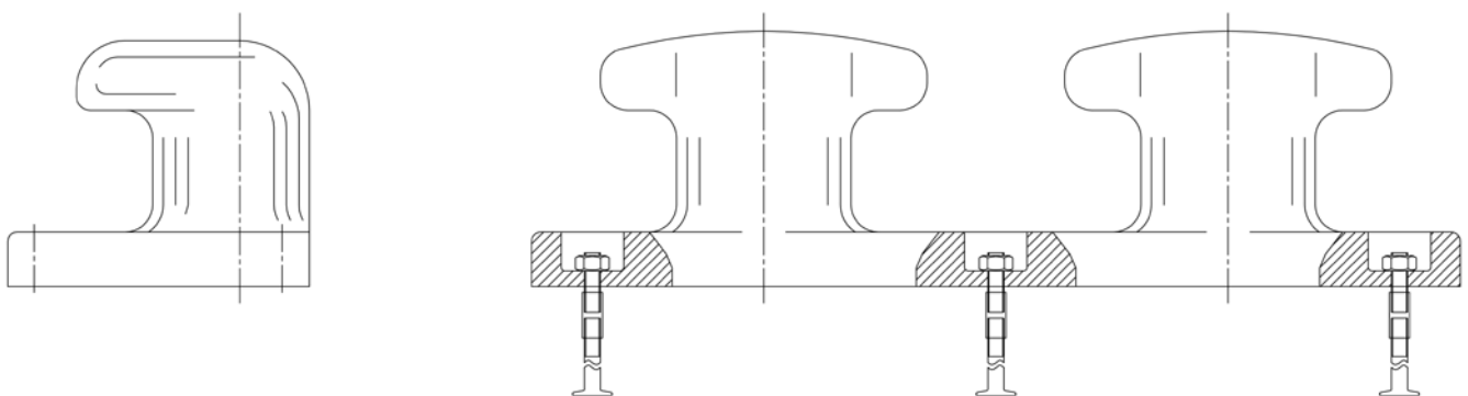
Double bollard
