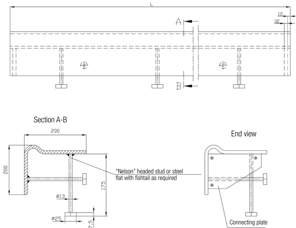
Horizontal protective nosing
