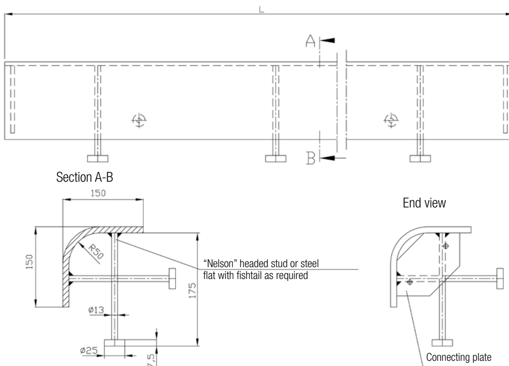
Vertical protective nosing
