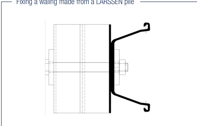
Fixing a waling made from a LARSEN pile
