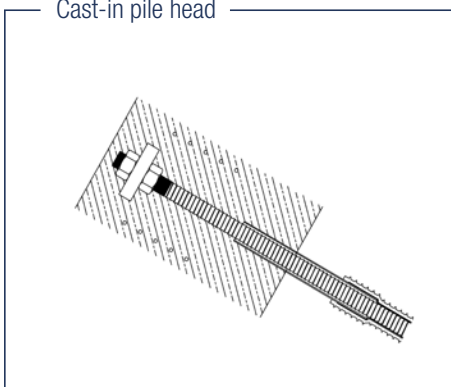
Cast-in pile head
