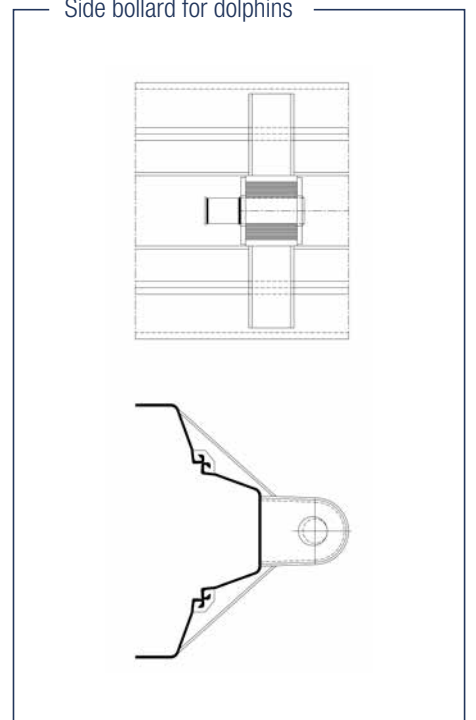
Side bollard for dolphins
