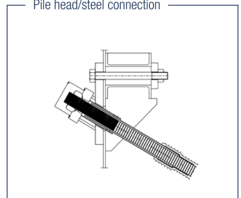
Pile head/steel connection
