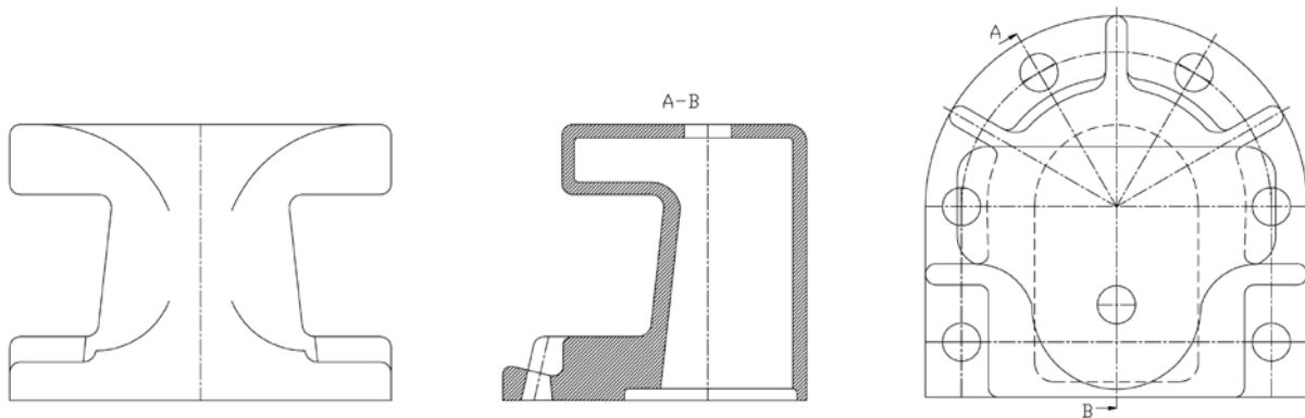
Single bollard
