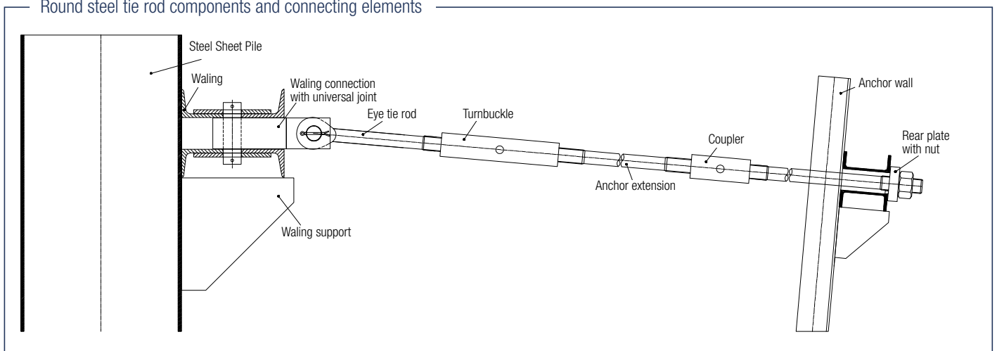
Round steel tie rod components and connecting elements
