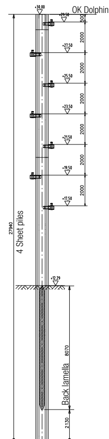
Elevation om breasting dolphin from water side
