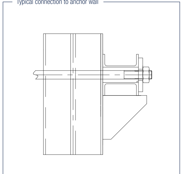
Typical connection to anchor wall
